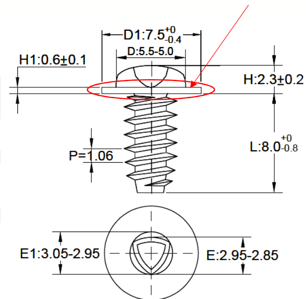
Screw with gasket
